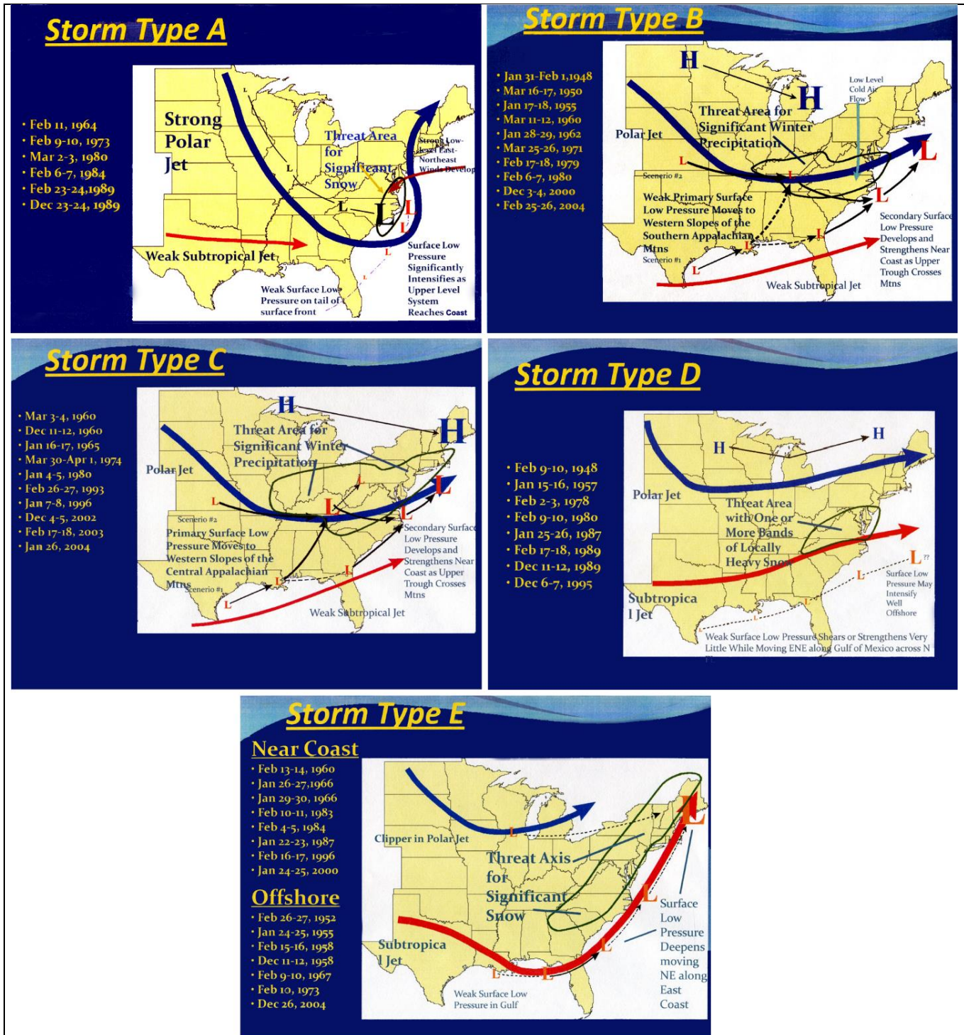
Figure 12-4. Nor'easter Miller Classifications
