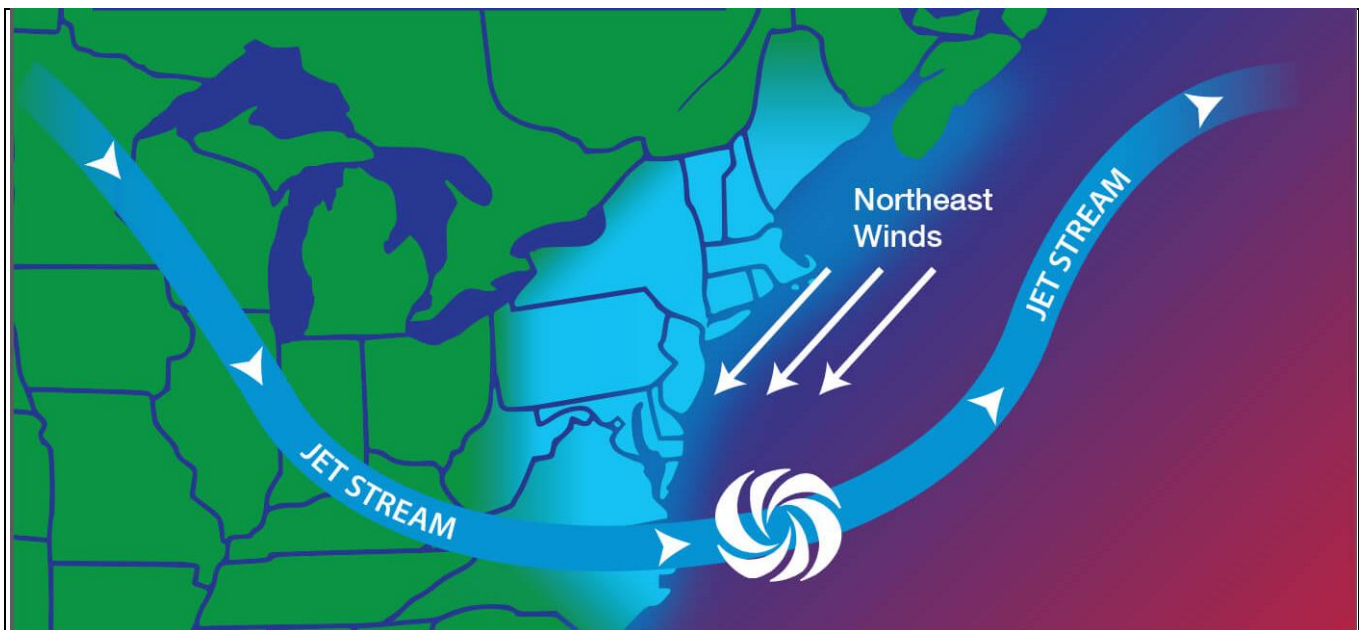
Figure 12-3. Formation of a Nor'easter
