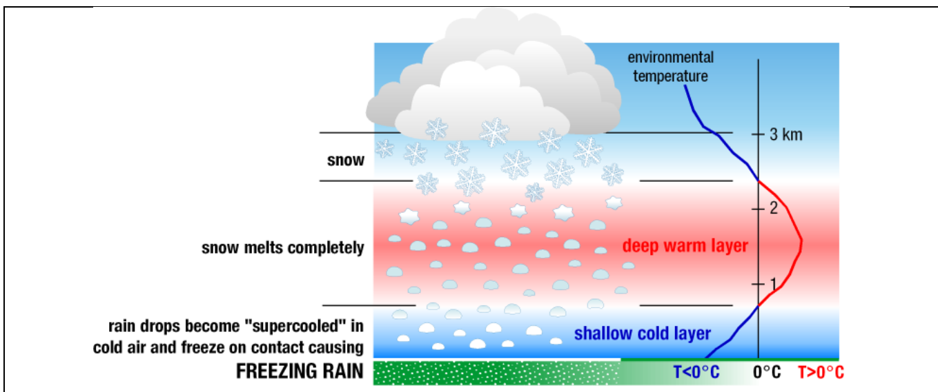
Figure 12-2. Freezing Rain Creation
