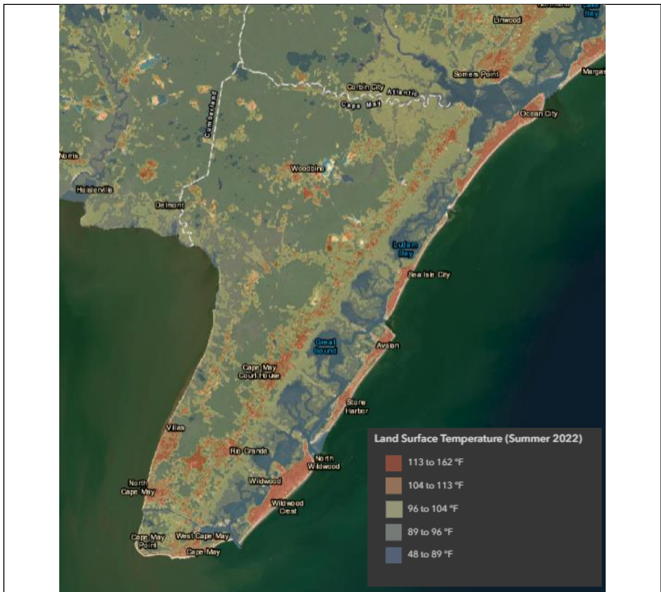
Figure 9-3. Urban Heat Island Effect and Land Surface Temperature in Cape May County
