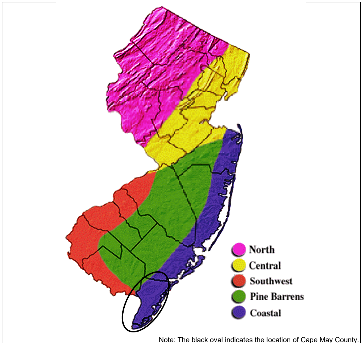
Figure 9-2. Climate Zones of the State of New Jersey
