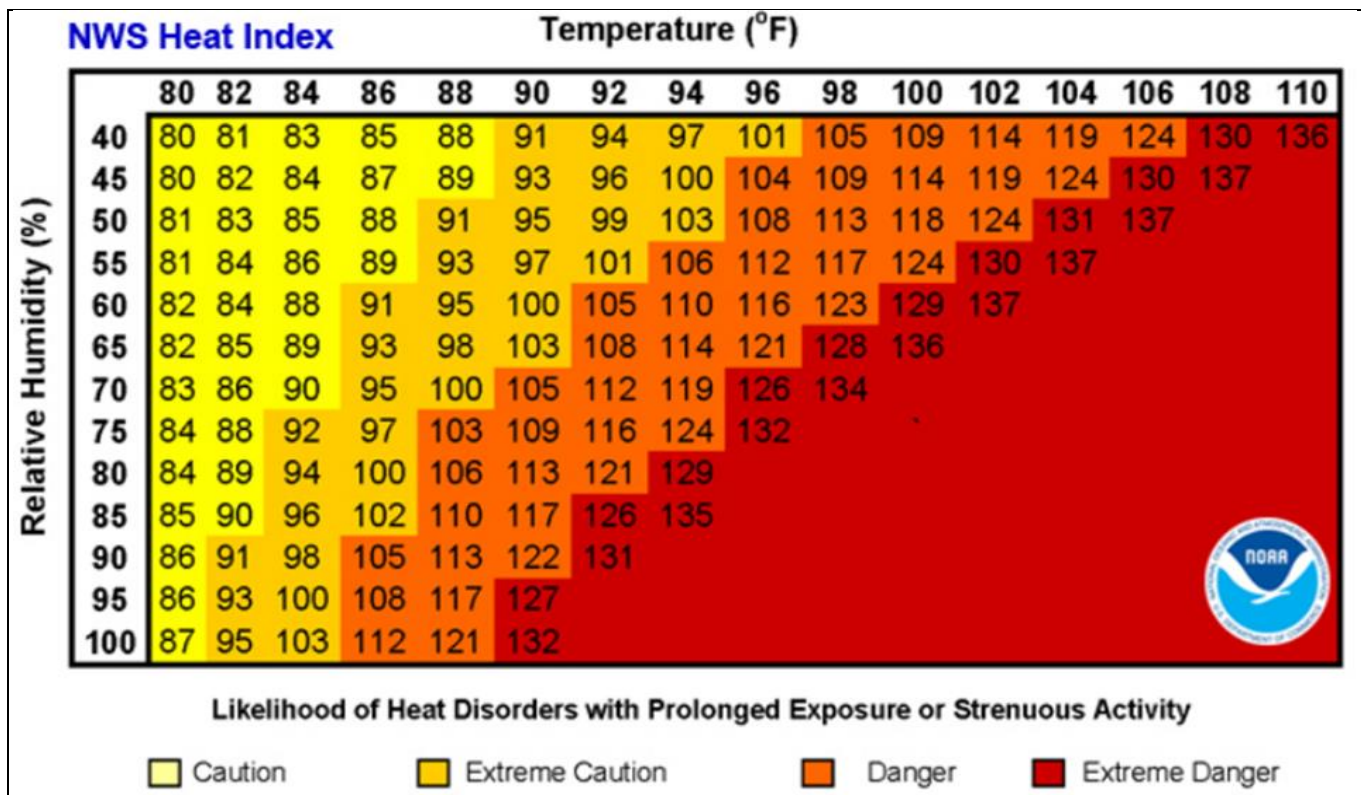
Figure 9-5. NWS Heat Index Chart – Shaded Areas
