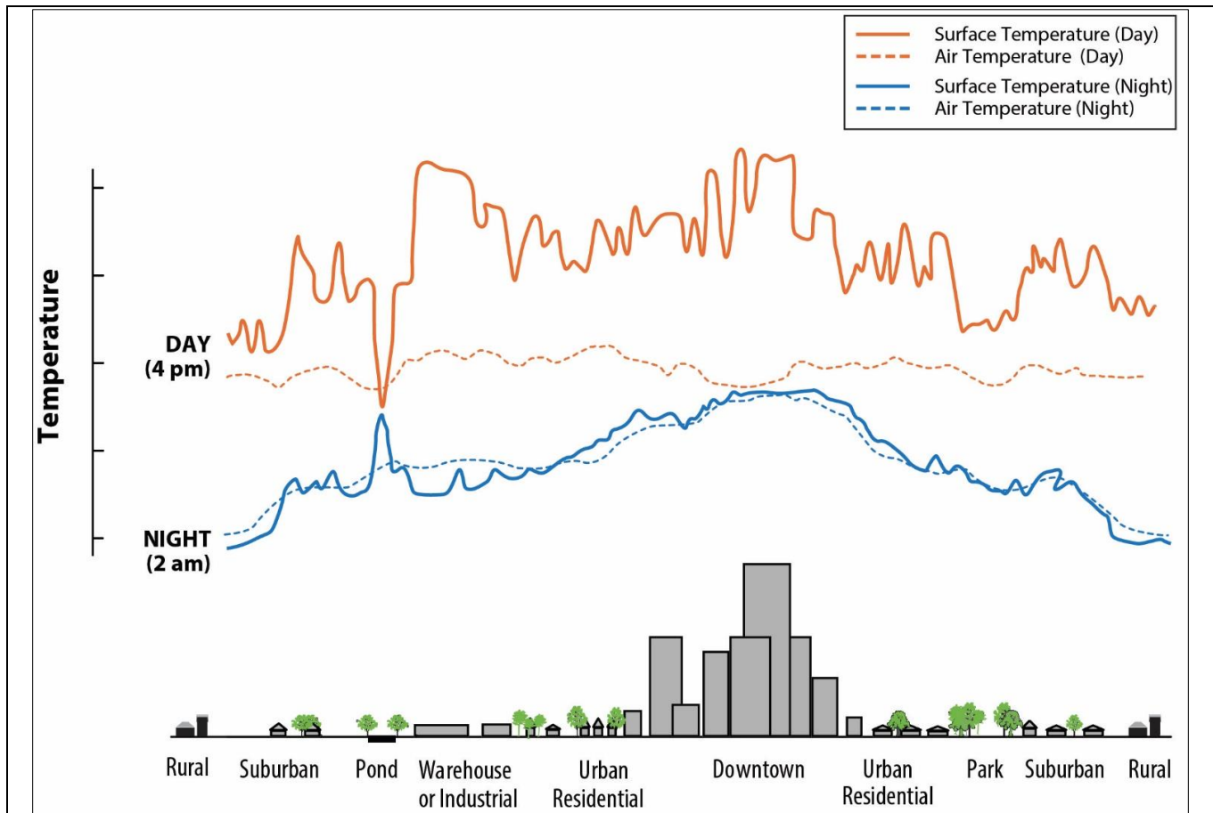
Figure 9-1. Urban Heat Island Effect Diagram
