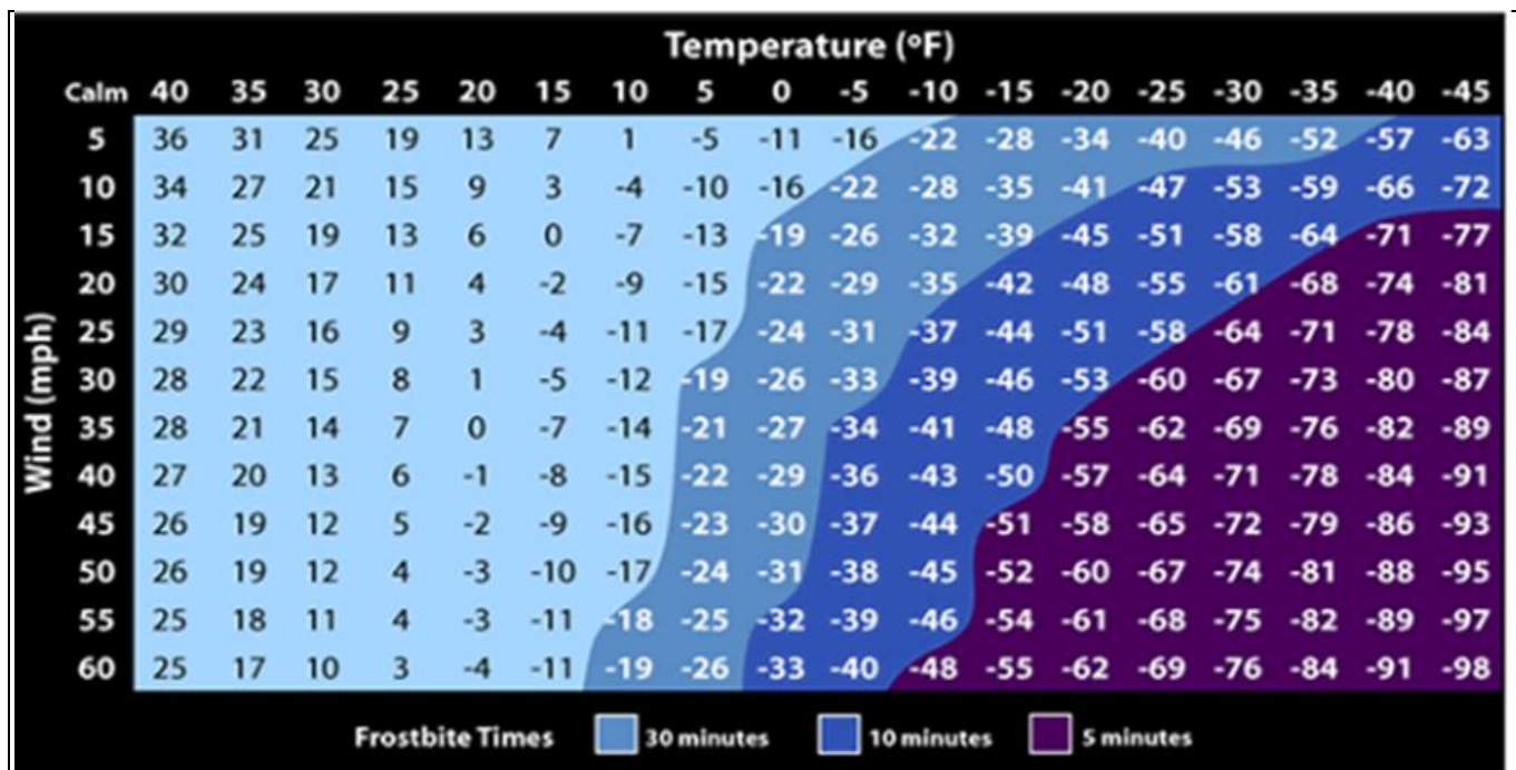
Figure 9-4. Wind Chill Index
